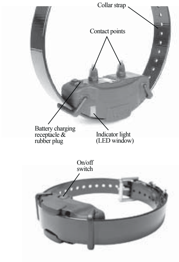
Receiver/Collar
